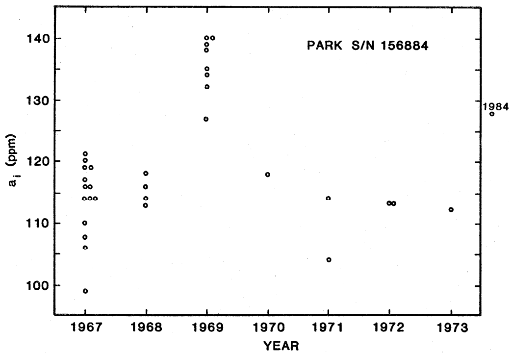
Figure 8. Measurements of a_i for Park resistor 156884 for the years 1967 to 1973.
