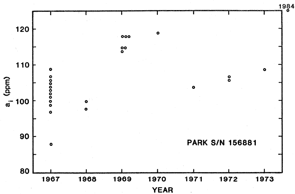
Figure 5. Measurements of a_i for Park resistor 156881 for the years 1967 to 1973.
