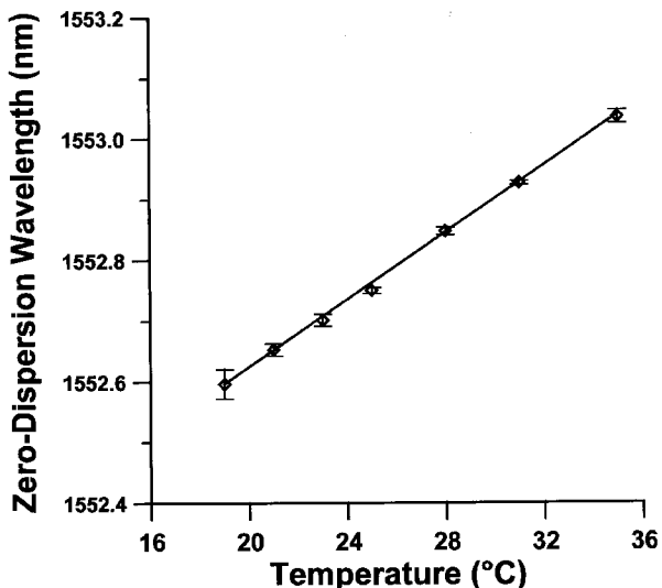
Fig. 12. The temperature dependence of \lambda_0 in a dispersion-shifted fiber. The slope of the line fitted to the data is +0.028 \text{ nm}/^\circ\text{C} . Error bars are 3 times the type A standard uncertainty for each data point.
